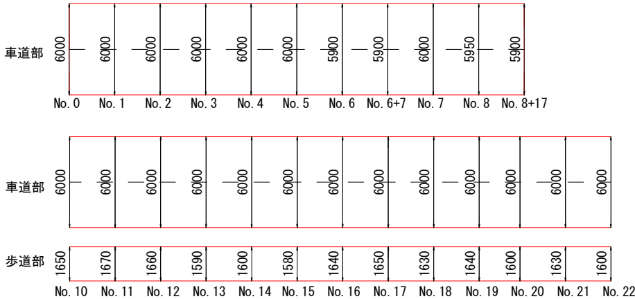
舗装展開図S=free
